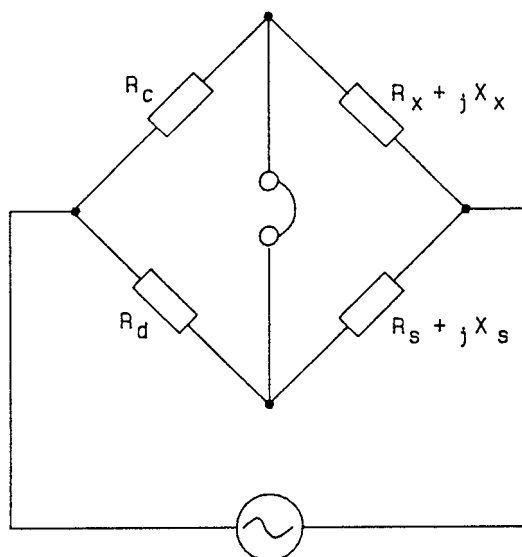
Figure 5-2—Similar-Angled Bridge
